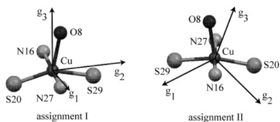
Figure 7. Two possible orientations of the principal axes of the g tensor for the Cu(II) site in [\text{Cu}(\text{ClO}_4)(\mathbf{L1})](\text{ClO}_4) . The direction cosines referred to the abc^* crystal axes are given in Table 3.
