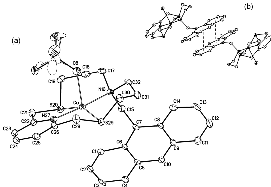
Figure 2. (a) Displacement ellipsoid representation (at the 40% probability level) of the [\text{Cu}(\text{ClO}_4)(\mathbf{L1})]^+ ion, with the atom-numbering scheme adopted. Noncoordinated counterions and hydrogen atoms were omitted for clarity. (b) Perspective view of dimers of [\text{Cu}(\text{ClO}_4)(\mathbf{L1})]^+ showing the \pi\cdots\pi interactions. Reproduced with permission from: Inorg. Chem. 2005 , 44 , 8105–8115. Copyright 2005 American Chemical Society.
