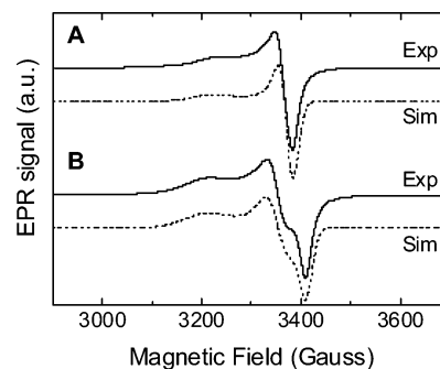
Figure 4. Experimental and simulated EPR spectra of powdered samples of (A) [\text{Cu}(\text{ClO}_4)(\text{L})](\text{ClO}_4) and (B) [\text{Cu}(\text{ClO}_4)(\text{L1})](\text{ClO}_4) , recorded at room temperature and 9.65 GHz. EPR simulations were performed using g_1 = g_2 = 2.043 (26), and g_3 = 2.145 (80) for [\text{Cu}(\text{ClO}_4)(\text{L})](\text{ClO}_4) and g_1 = 2.025 (26), g_2 = 2.060 (34), and g_3 = 2.155 (80) for [\text{Cu}(\text{ClO}_4)(\text{L1})](\text{ClO}_4) . Line widths are in gauss in parentheses.
